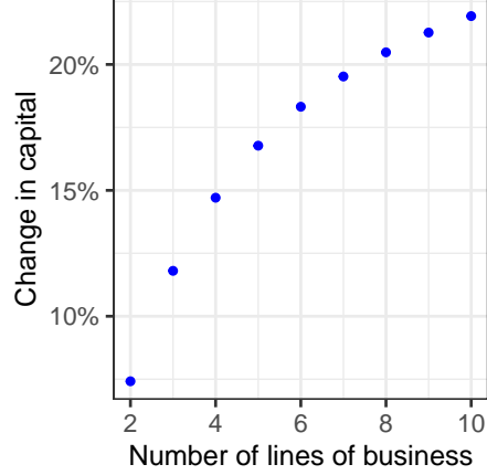
Figure 3: The maximal changes in the diversified capital for multiple lines of business if we increase the correlations from \rho = 0.3 to p = 0.5 for n = 2, \dots, 10 lines of business.
