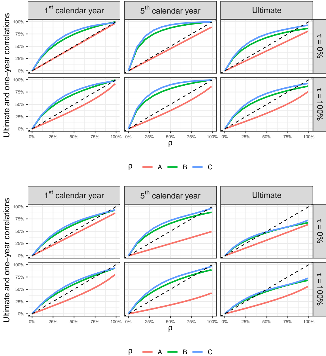
Figure 6: The one-year correlations in future calendar years and the ultimate correlations (solid lines) as a function of \rho , together with the diagonal (dotted lines) - lines 4 and 7 (top) and lines 4 and 12 (bottom).
