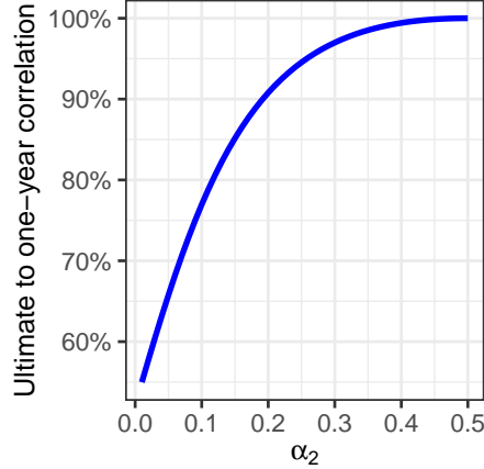
Figure 1: The ratio of the ultimate correlation (3.3) to the one-year correlation (3.4) under the volatility parameters specified with (3.7).
