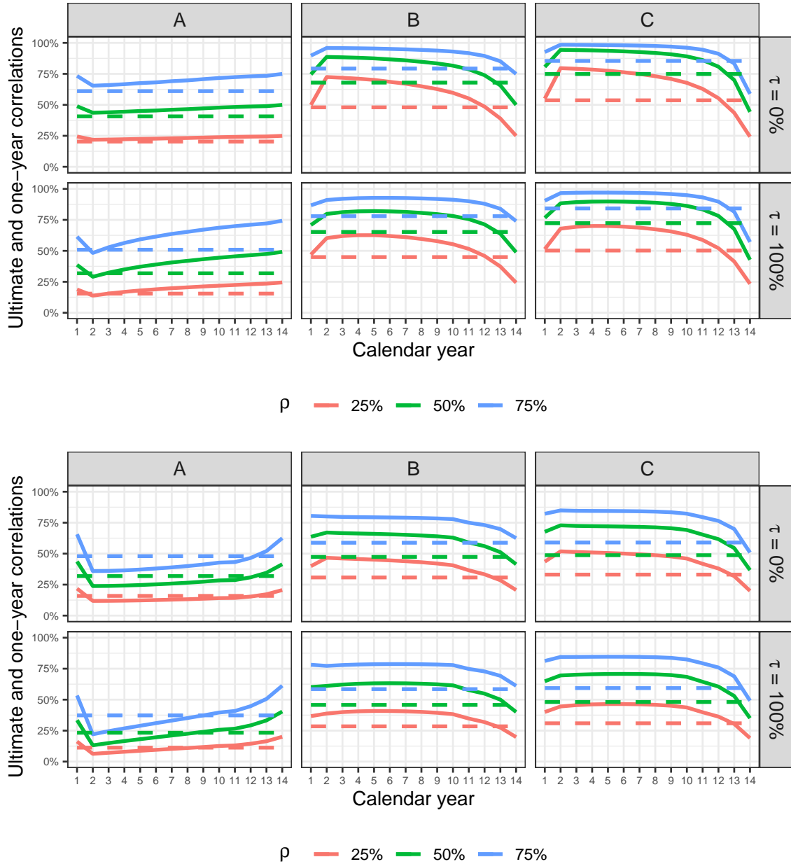
Figure 5: The one-year correlations in future calendar years (solid lines) and the ultimate correlations (dotted lines) - lines 4 and 7 (top) and lines 4 and 12 (bottom).
